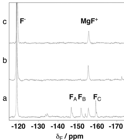
Fig. 2. 19 F NMR spectra of the MgF 3 − / \beta -PGM system. (a) The peaks labeled F A -C (−147, −152, and −159 ppm) correspond to MgF 3 − bound to \beta -PGM in the presence of G6P. [NH 4 F] = 10 mM, [MgCl 2 ] = 5 mM, [ \beta -PGM] = 1 mM, [G6P] = 5 mM. Conditions: pH 7.2, [K + Hepes] = 50 mM, 5°C. (b) Control with G6P omitted. (c) Control with G6P and \beta -PGM omitted. The peak at −119 ppm is free fluoride in solution (F − ), and the peak at −156 ppm is MgF + . The three 19 F resonances (−134, −135, and −154 ppm), with \approx 10% of the intensity of the major peaks, most likely correspond to a minor conformer of the MgF 3 -TSA complex that exchanges with the major conformer more rapidly than the complex dissociates, because these resonances correlate via saturation transfer with specific resonances of the major conformer (resonances F A , F B , and F C , respectively).
