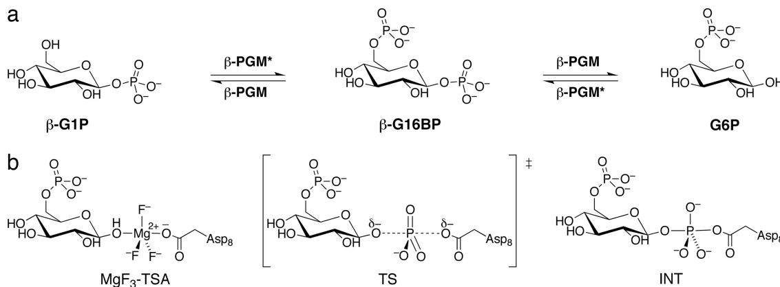
Fig. 1. The reaction mechanism of \beta -PGM and the potential enzyme stabilized species. (a) \beta -PGM catalyzes the interconversion of \beta -glucose-1-phosphate ( \beta -G1P) and \beta -glucose-6-phosphate (G6P) via \beta -glucose-1,6-bisphosphate ( \beta -G16BP) and the phosphorylated form of the enzyme ( \beta -PGM*). (b) The TS for the latter part of the \beta -PGM catalyzed reaction (i.e., \beta -G16BP to G6P), the proposed phosphorane INT and the TSA (MgF 3 -TSA) formed from \beta -G6P, magnesium, and fluoride.
