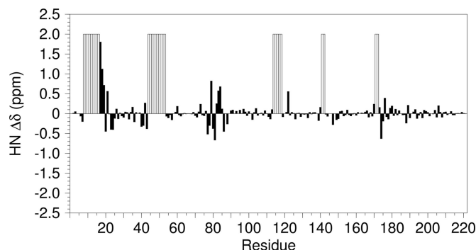
Fig. 3. Histogram of backbone amide proton chemical shift changes ( \Delta\delta ) plotted against residue between \beta -PGM in the open form and \beta -PGM in \text{MgF}_3\text{-TSA} . Positive \Delta\delta represent up-field changes for the open to closed transition. Large \Delta\delta are expected in regions of \beta -PGM involved in binding substrate in the active site. However, no data were obtained for residues in the active site loops (D8–T16, L44–L53, S114–N118, V141–A142, and S171–Q172) in the open conformation, because the corresponding ^{15}\text{N} -TROSY peaks were broadened beyond the limits of detection. This line-broadening behavior is indicative of a conformational dynamics process between two (or more) similarly populated forms, and the difference in ^1\text{H} chemical shift of \approx 2 ppm between these interconverting conformations equates to conformational dynamics occurring in the millisecond timescale (i.e., dynamics in the intermediate exchange regime for ^1\text{H} ). These residues are depicted with open bars. Further significant \Delta\delta involve residues A17–Q43 positioned in two \alpha -helices of the “cap” domain and N77–S88, which locate to the C-terminal portion of the S65–I84 \alpha -helix and the “hinge” region (Q85–Y93). For the remainder of \beta -PGM, small \Delta\delta indicate that, on formation of \text{MgF}_3\text{-TSA} , there is little change in the local protein fold outside of these regions.
